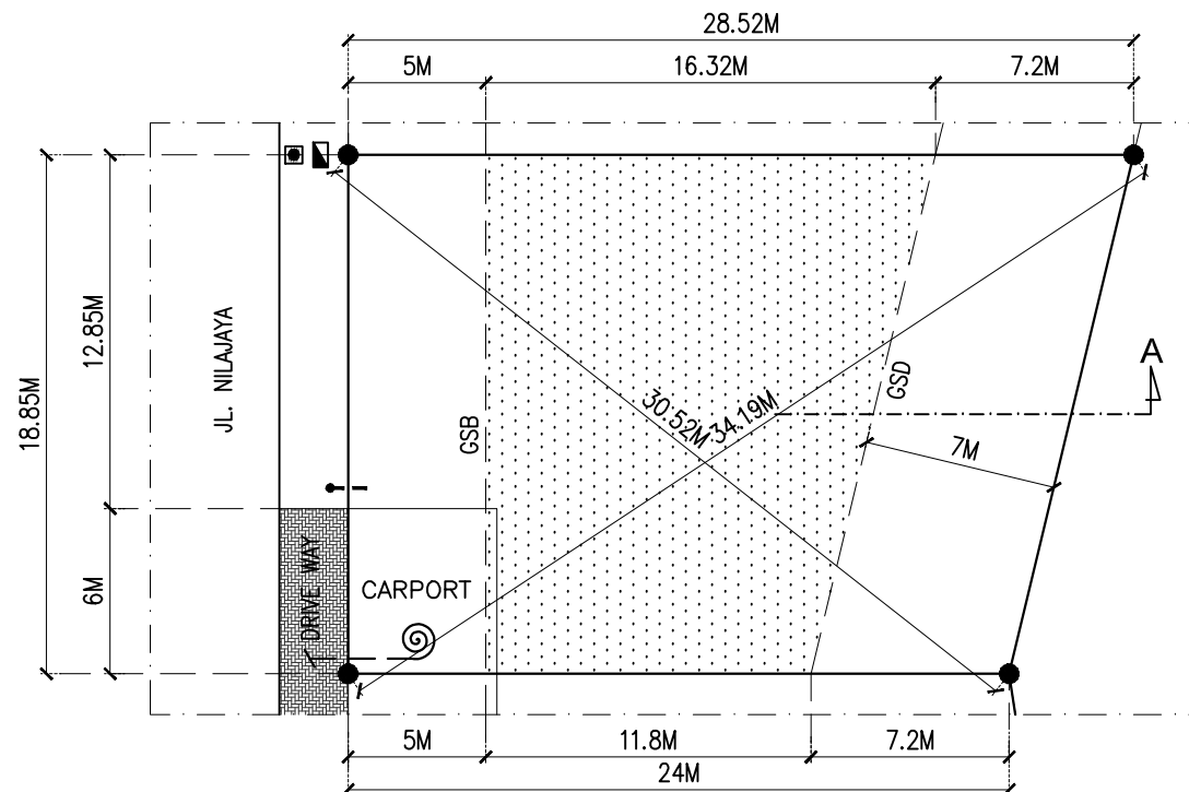
DENAH KAVLING JL. NILAJAYA NO. 39 SKALA 1 : 300
